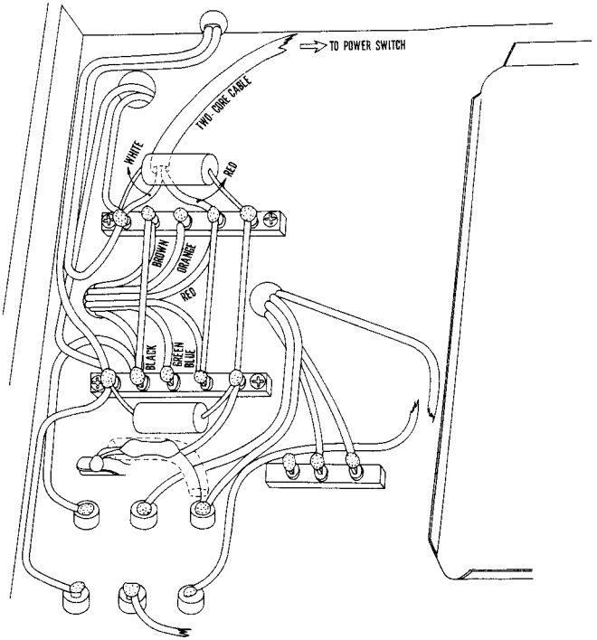
SCHEMATIC FOR 117V OPERATION
